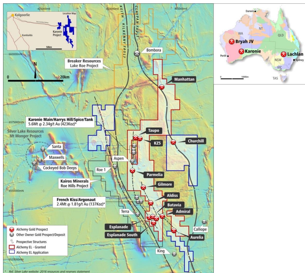
Figure 1: Karonie Project tenements, major deposits, prospects and interpreted major structures over aeromagnetic image
