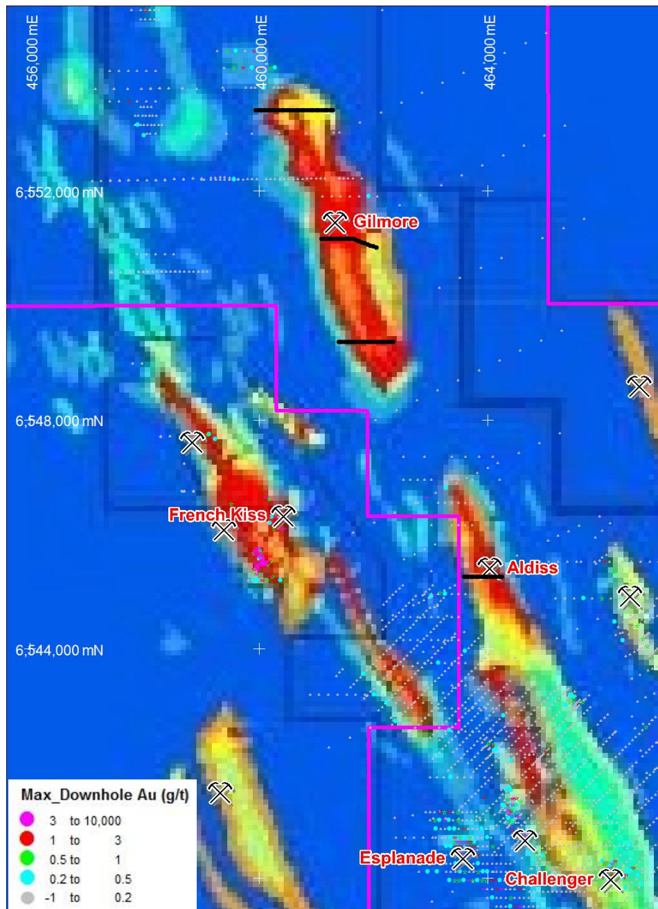
Figure 2: Karonie Project proposed aircore drill lines (black), tenement outline (pink), and prospects over combined evidence weighted probability map (modified from open file SRK report “Prospectivity Study for the Aldiss Project Area” dated December 2014)
