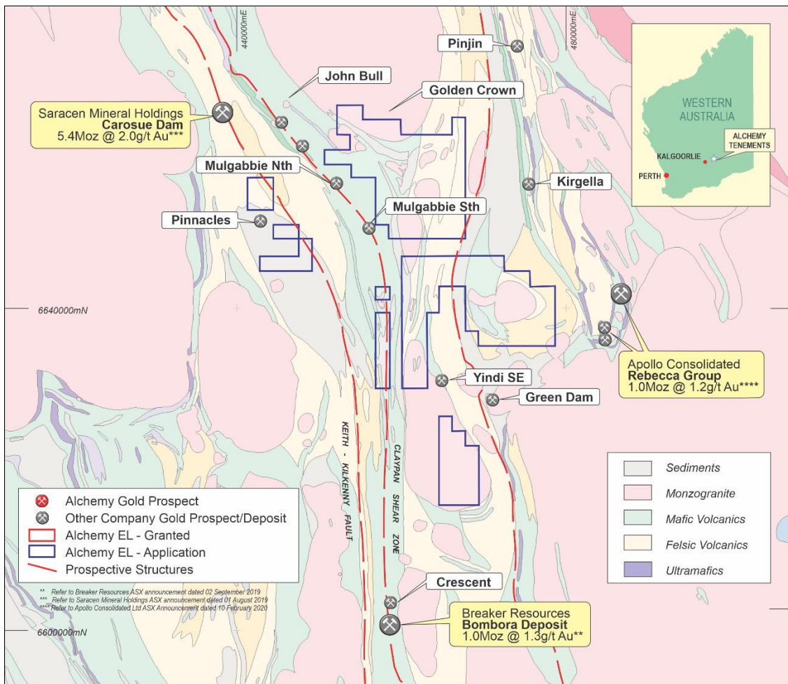
Figure 2: Lake Rebecca Project tenements, prospects and interpreted structures over 250K geology
