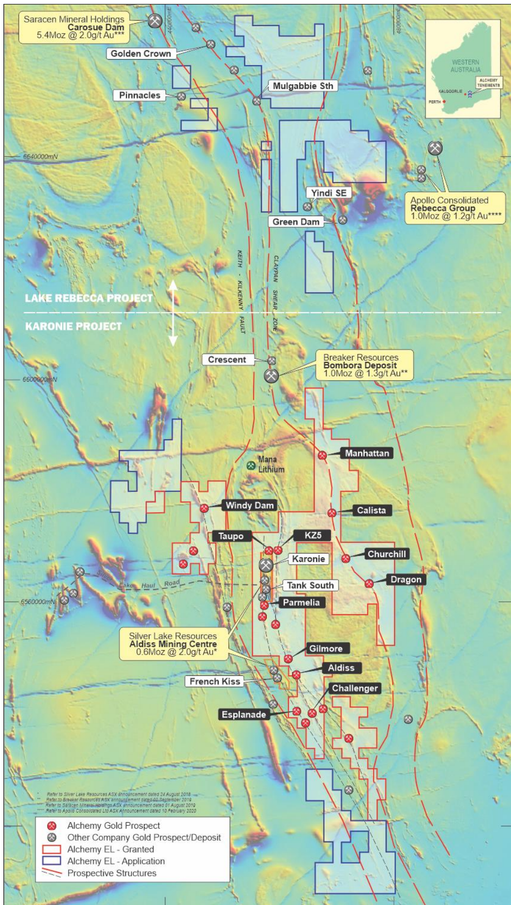
Figure 1: Lake Rebecca and Karonie Projects: tenements, prospects and interpreted structures over aeromagnetic image
