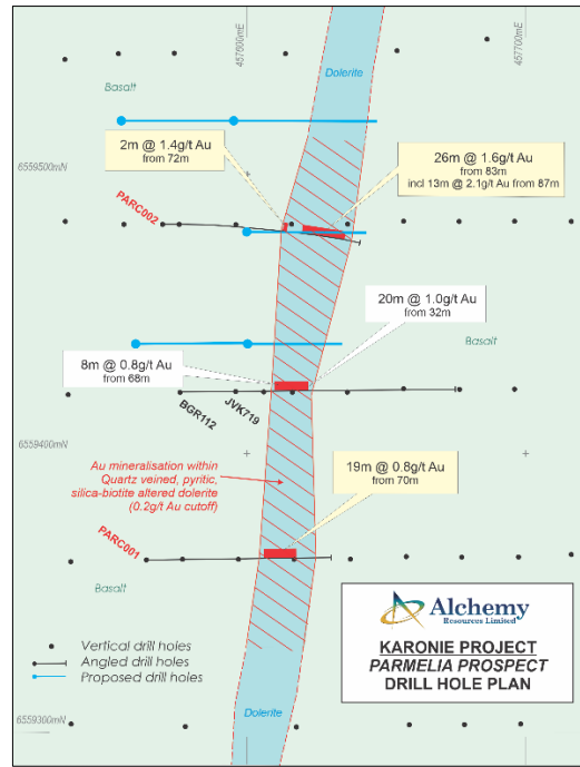
Figure 2: Parmelia prospect proposed RC drilling and previous drilling over interpreted geology
