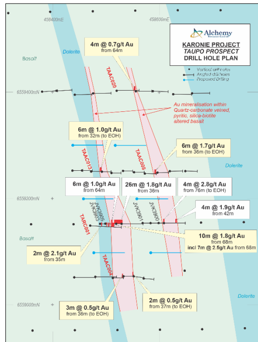
Figure 3: Taupo prospect proposed RC drilling and previous drilling over interpreted geology
